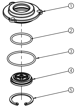
②⑧ PART NO. 7106709 CRANKCASE SIGHTGLASS KIT
